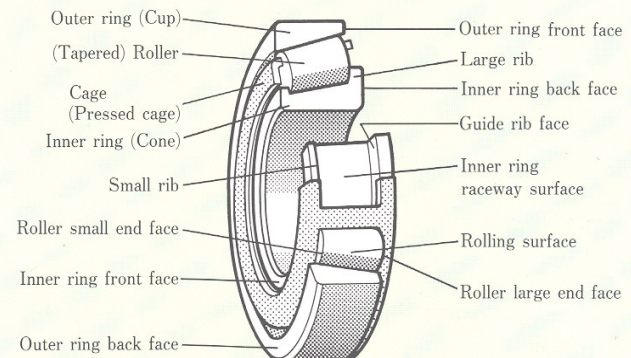
(c) Tapered roller bearing
