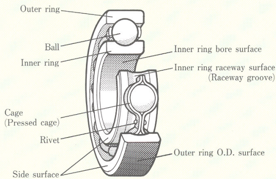
(a) Deep groove ball bearing
