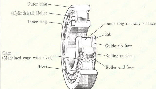
(b) Cylindrical roller bearing
